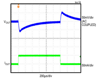
LOAD CURRENT TRANSIENT RESPONSE ( V_{IN} = 24V , V_{OUT} = 3.3V , I_{OUT} = 0A TO 0.05A )
