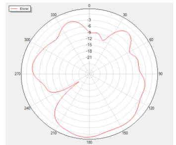
Theta=90 Freq=4000MHz
