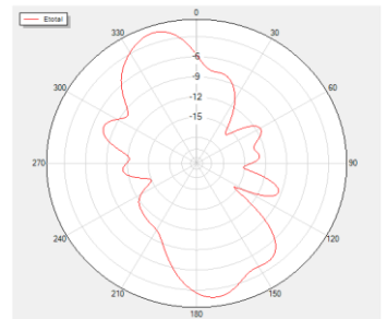
Theta=90 Freq=5500MHz
