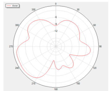
Phi=90 Freq=4000MHz
