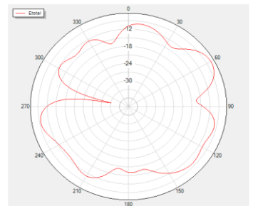
Phi=90 Freq=5500MHz
