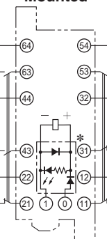
G7SA-3A3B Mounted
