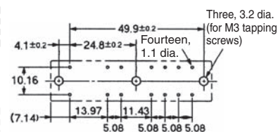
G7SA-4A2B Mounted
