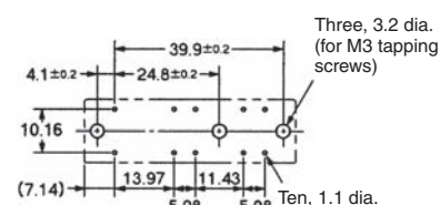
G7SA-2A2B Mounted
