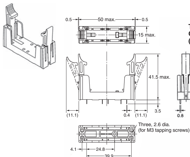
G7SA-3A1B Mounted
