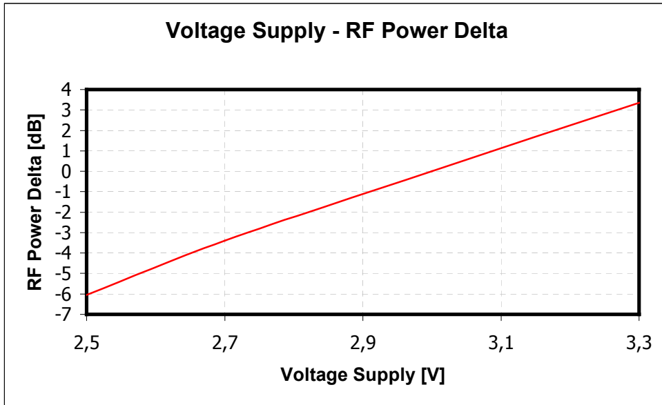
Fig. 3 RF Power (E.R.P.) delta Vs Voltage Supply
