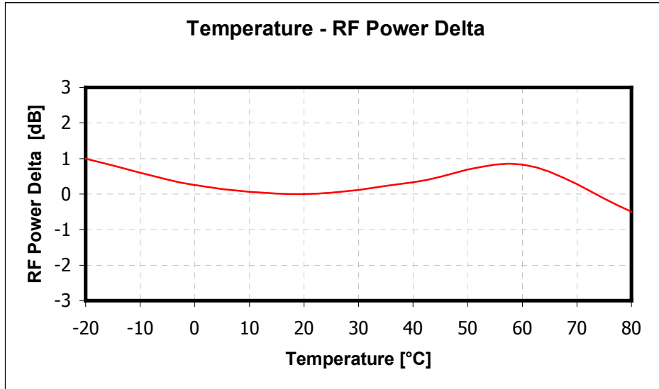
Fig. 5 RF Power (E.R.P.) delta Vs Temperature
