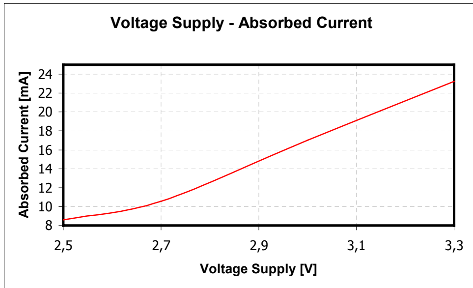
Fig. 4 Absorbed current Vs Power Supply
