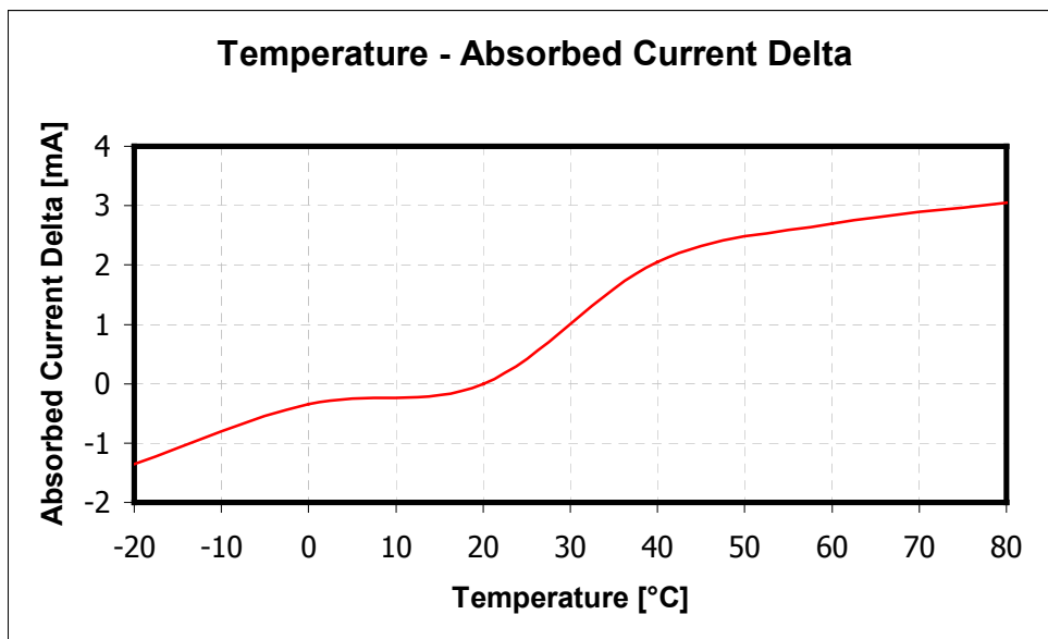
Fig. 6 Absorbed current delta Vs Temperature
