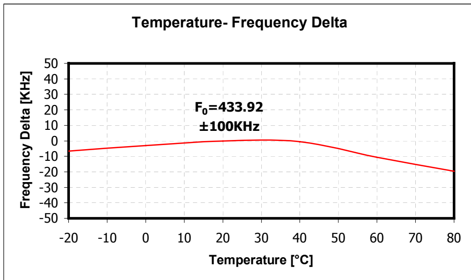
Fig. 7 Frequency delta Vs Temperature
