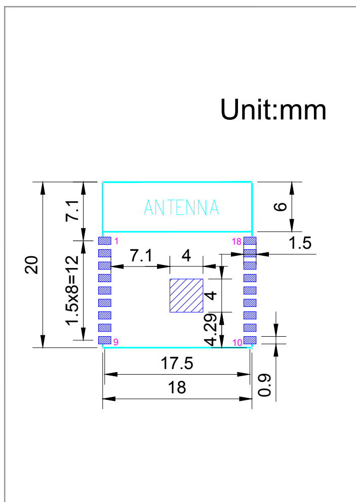
Figure 8-1. Recommended PCB Land Pattern of ESP-WROOM-02D
