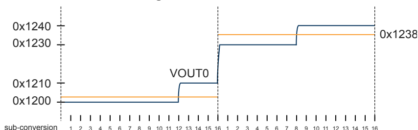
Figure 44-5. DAC Conversions in Dithering Mode
