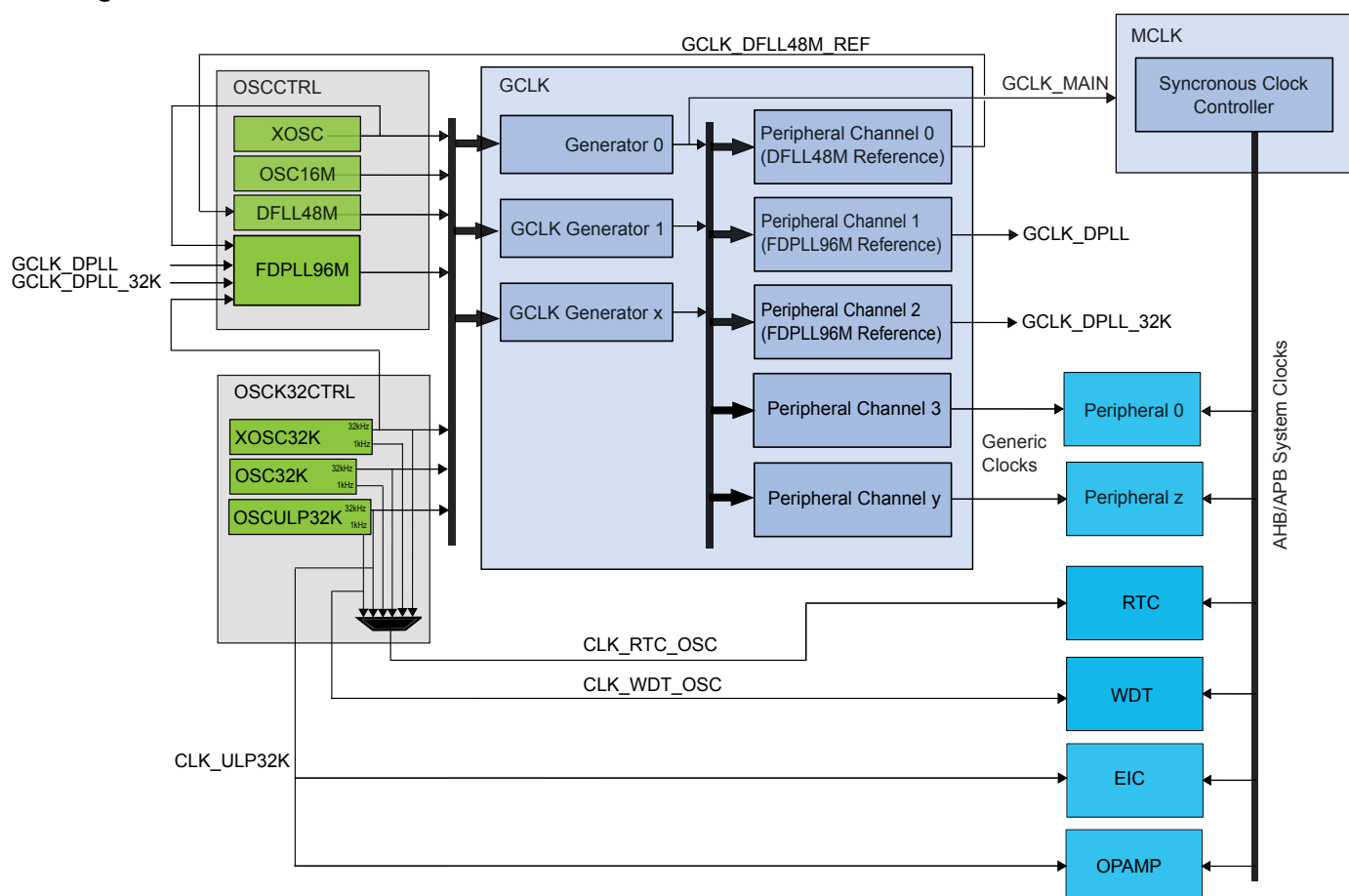
Figure 16-1. Clock Distribution
