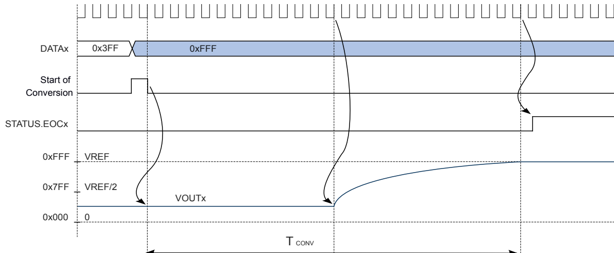
Figure 44-2. Single DAC Conversion
