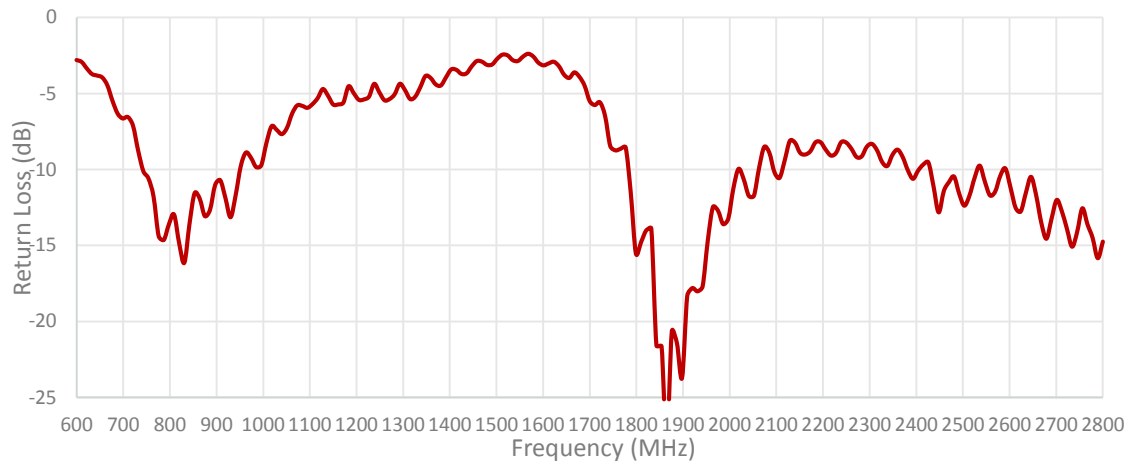
Cable 1: CELLULAR/LTE
