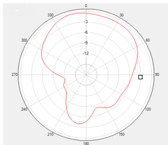
Phi=0 Freq=1176MHz
