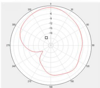
Phi=0 Freq=1602MHz
