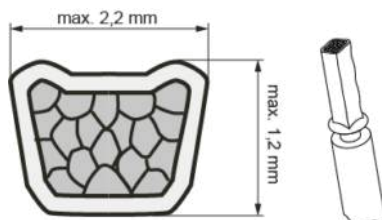
Fig. 1: Trapezoid crimp
