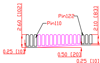
Detail D
