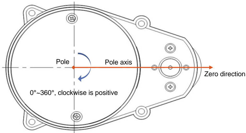
FIG 3 YDLIDAR X4 POLAR COORDINATE SYSTEM DEFINITION
