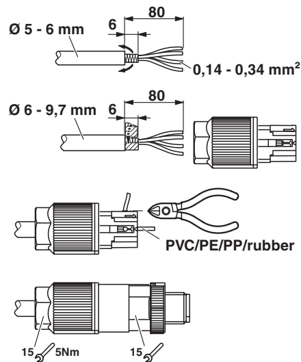
Functional drawing
