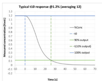
Typical recovery time (from 1.2% Propane)
