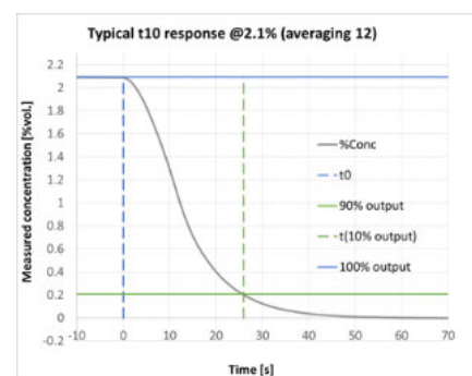
Typical recovery time (from 2.1% Propane)
