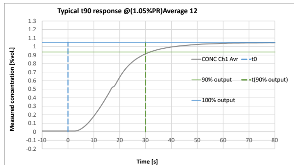
Typical T90 Response Time without Dust Filter (to 1.05% Propane)
