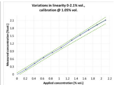
Typical Linearity 0-2.1% Propane
