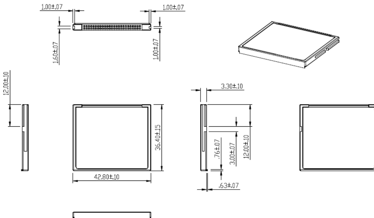
Figure 7-1: Physical Dimensions
