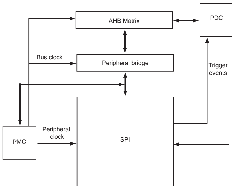
Figure 33-1. Block Diagram
