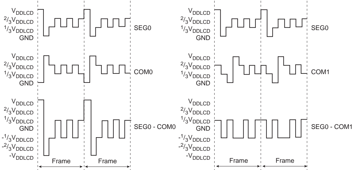
Figure 39-6. Driving an LCD with Four Common Terminals
