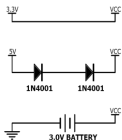
Figure 2: Power Supply Options
