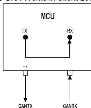
Figure 105 CAN Works in Silent Loopback Mode
