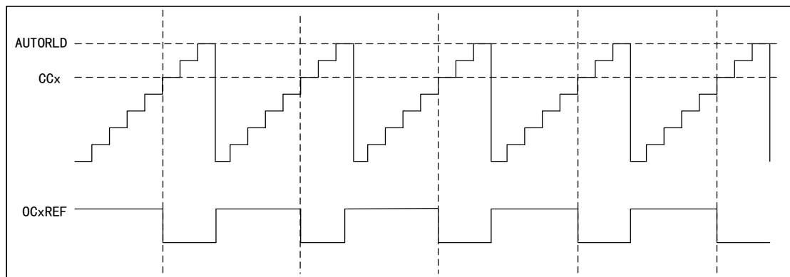
Figure 26 PWM1 Count-up Mode Timing Diagram
