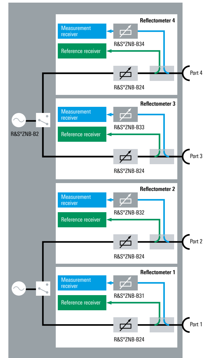
Block diagram of an R&S®ZNB 4-port model with two internal sources
