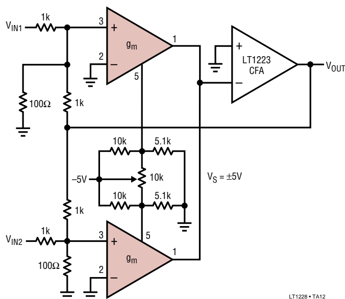
Video Fader
