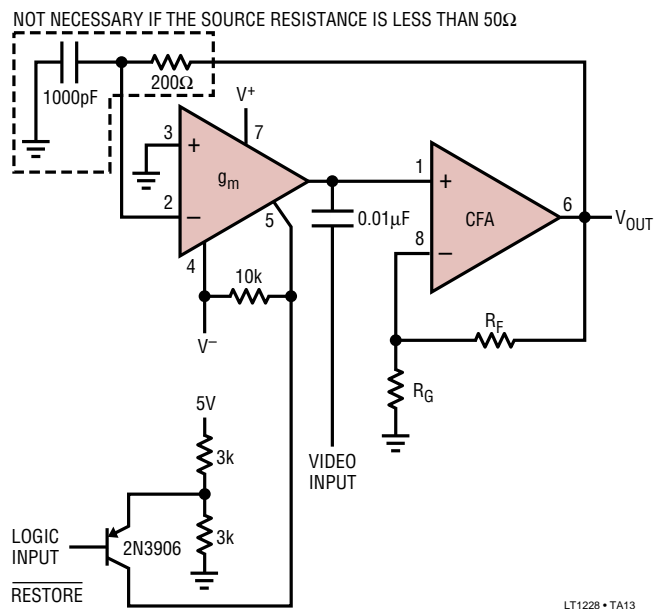
Video DC Restore (Clamp) Circuit
