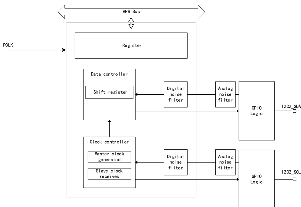
Figure 106 I2C2 Function Structure Diagram
