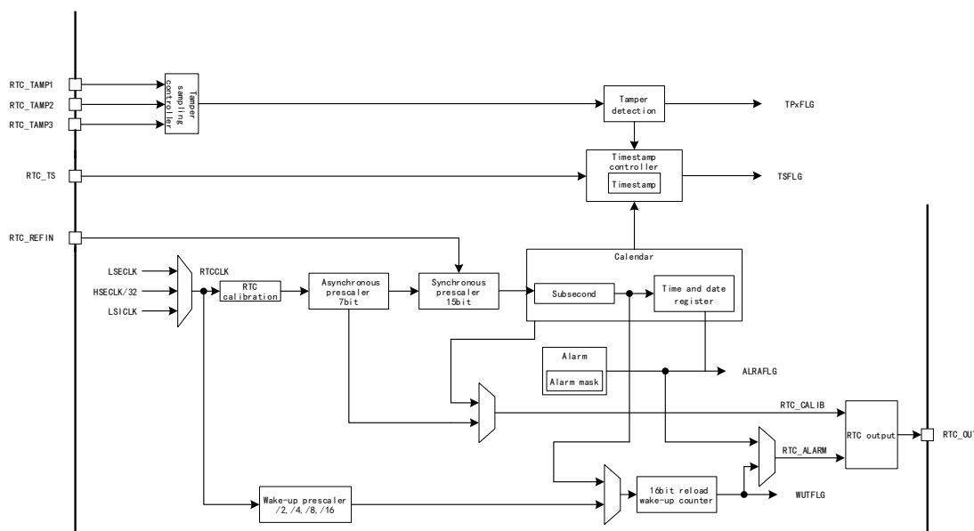
Figure 92 RTC Structure Block Diagram
