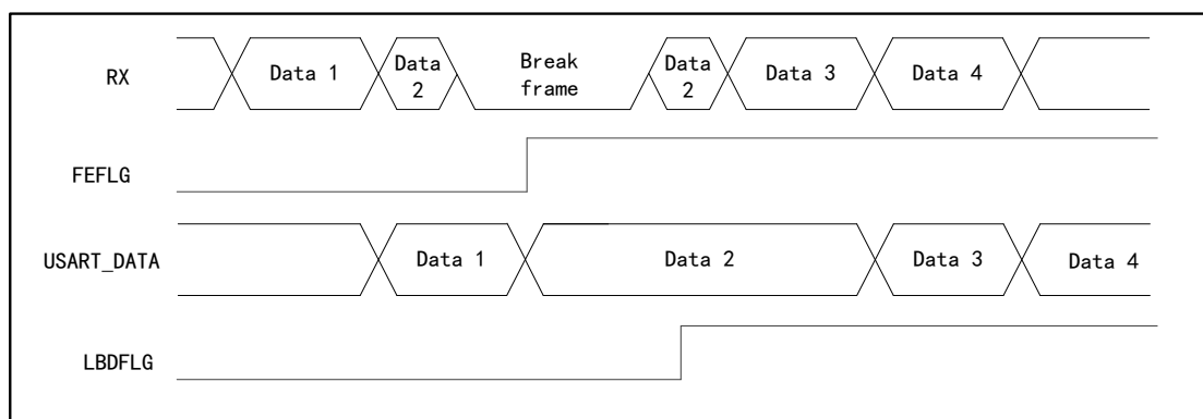
Figure 100 Break Frame Detection in Data Transmission State
