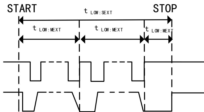
Figure 110 t_{\text{LOW:SEXT}} and t_{\text{LOW:MEXT}} Time
