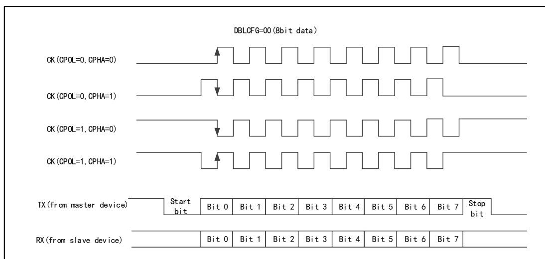
Figure 97 USART Synchronous Transmission Timing Diagram (DBLCFG=00)
