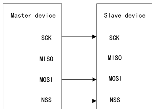
Figure 114 Connection in Simplex Mode (the master only transmits, while the slave receives)
