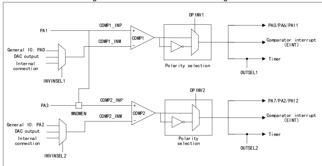
Figure 140 COMP Structure Block Diagram
