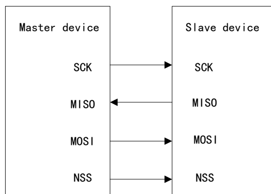
Figure 112 Connection in Half Duplex Mode
