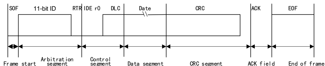
Figure 126 Standard Data Frame
