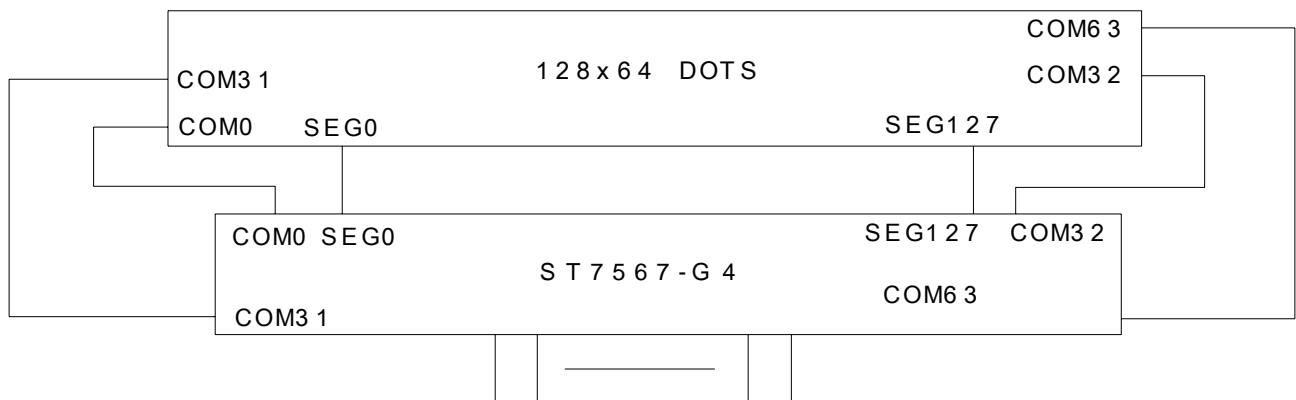
Figure 1 . Block Diagram
