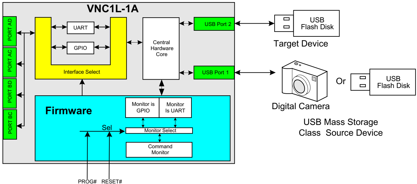
Figure 4 - DF2FC Firmware model
