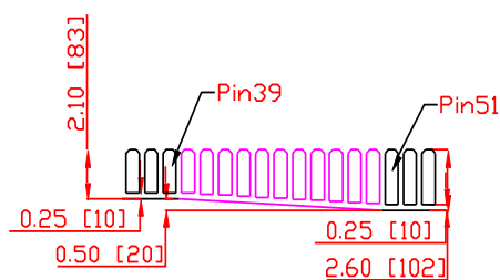
Detail C
