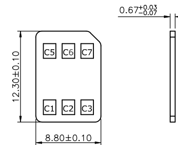
nano SIM dimensions
