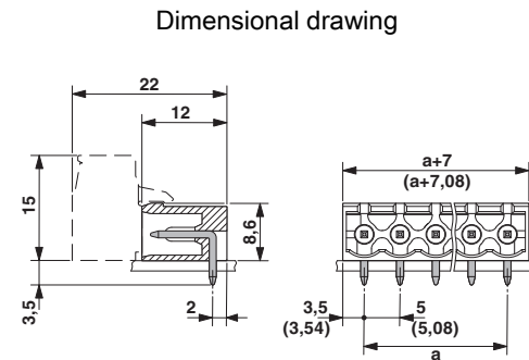
Type: ICV 2,5/...-G-5,08 with MSTBA 2,5/...-G-5,08
