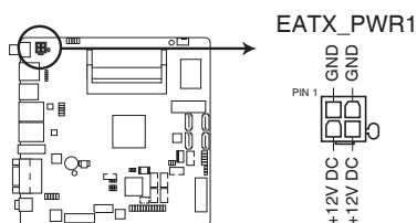
EMB-BT1 12VDC power connector
