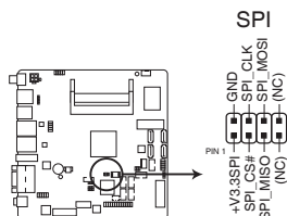
EMB-BT1 BIOS Programmable Connector
