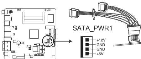
EMB-BT1 SATA POWER Connector
