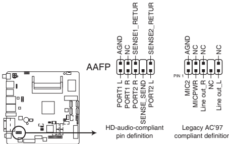
EMB-BT1 Front panel audio connector
