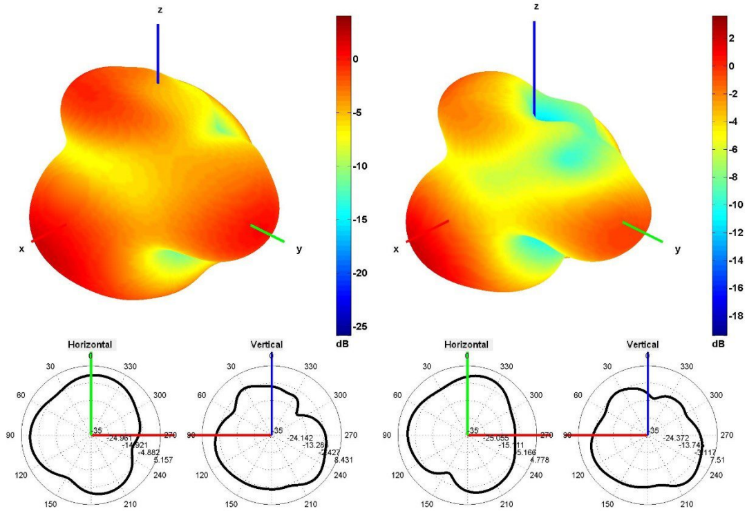
860 and 920 MHz Radiation pattern
