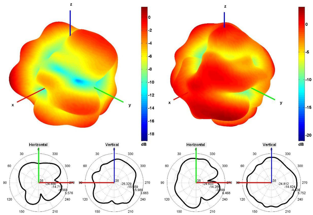
1950 and 2110 MHz Radiation pattern
