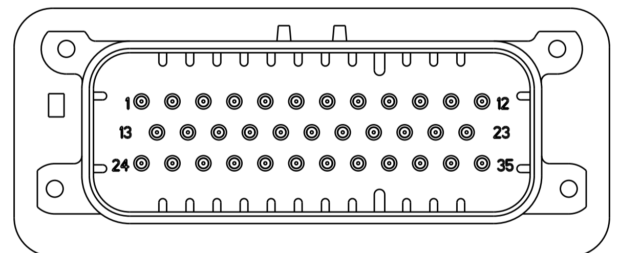
776230-4 & 1-776230-4 KEY LOCATION SCALE 2:1
