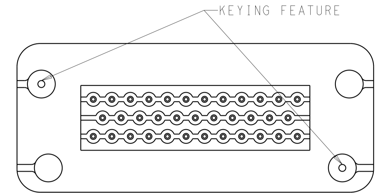
KEYING FOR 776230-1, 1-776230-1, 776230-4, 1-776230-4 AND 1-776230-6 SCALE 2:1
