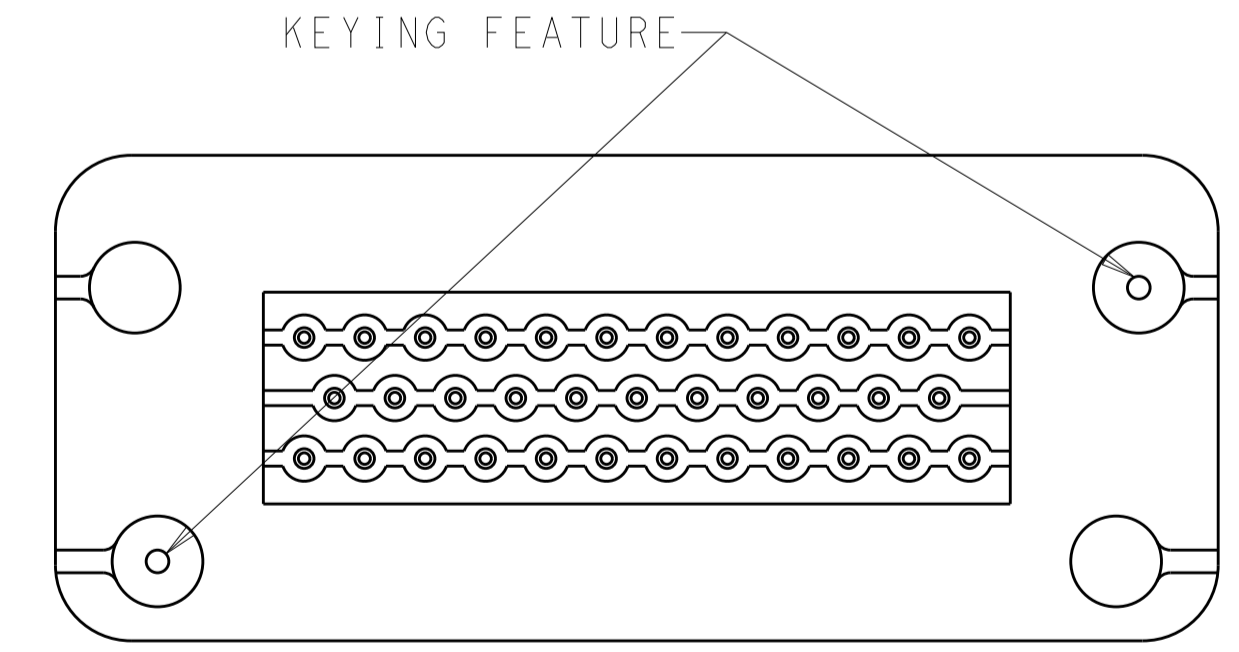
KEYING FOR 776230-2, 1-776230-2, 776230-5 AND 1-776230-5 SCALE 2:1
