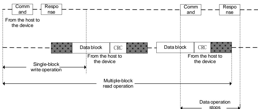
Figure 122 SDIO "Multi-" Data Block Write Operation
