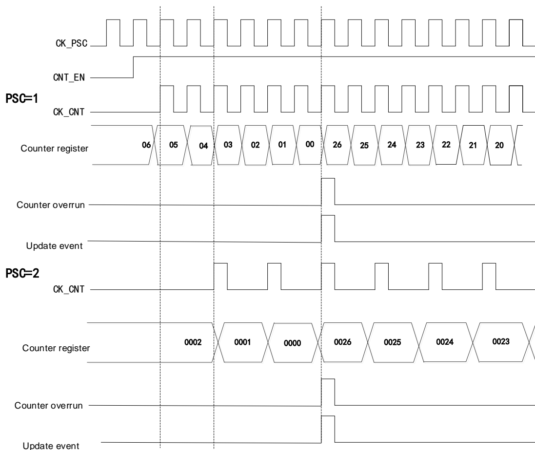
Figure 26 Timing Diagram when Division Factor is 1 or 2 in Count-down Mode
