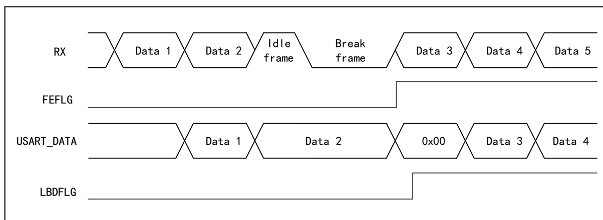
Figure 72 Break Frame Detection in Idle State
