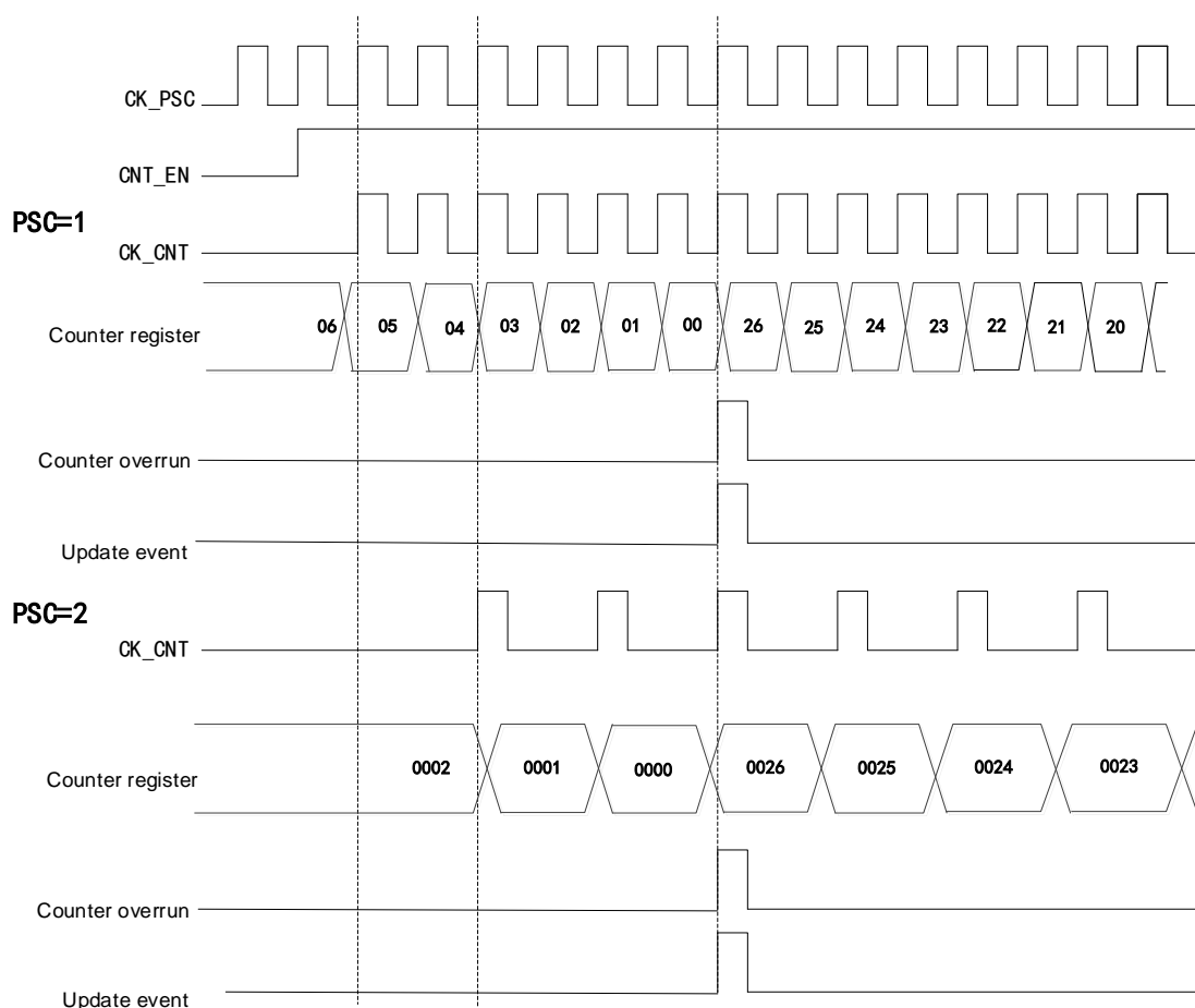
Figure 47 Timing Diagram when Division Factor is 1 or 2 in Count-down Mode
