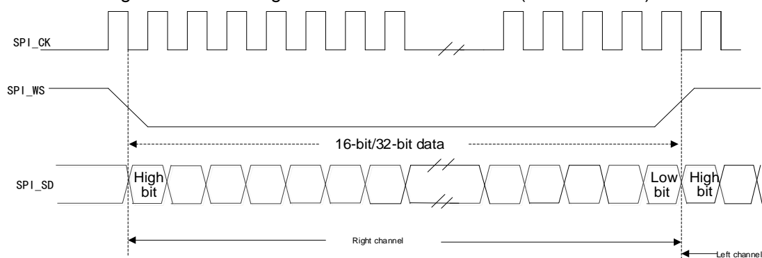
Figure 102 MSB Alignment Standard Waveform (16/32-bit data)
