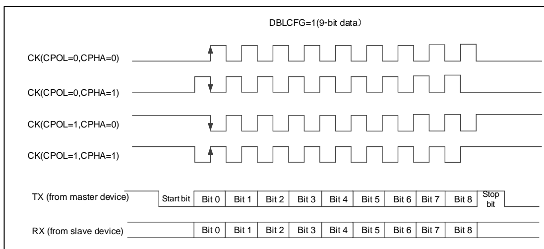
Figure 71 USART Synchronous Transmission Timing Diagram (DBLCFG=1)
