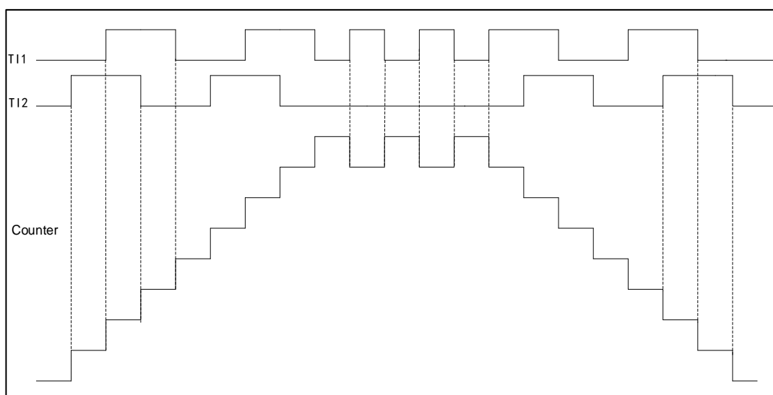
Figure 57 Counter Operation Example in Encoder Mode
