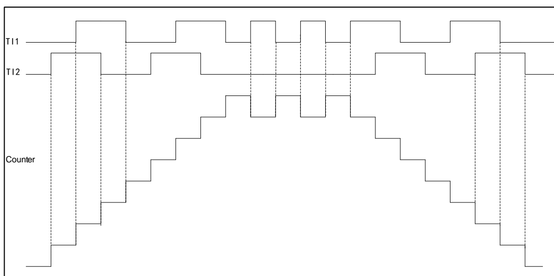
Figure 40 Counter Operation Example in Encoder Mode
