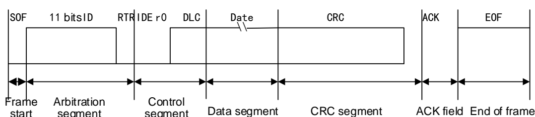
Figure 110 Standard Data Frame
