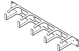
ISOMETRIC
