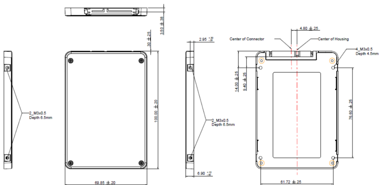
Figure 7-1 Physical Dimensions
