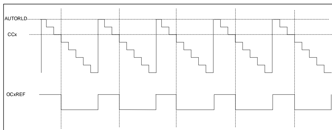
Figure 76 PWM2 Count-down Mode Timing Diagram
