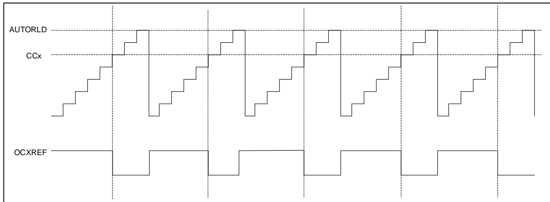
Figure 55 PWM1 Count-up Mode Timing Diagram
