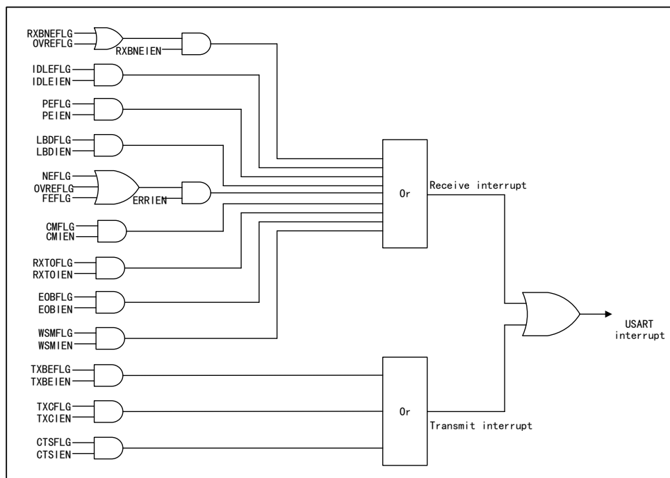
Figure 102 USART Interrupt Mapping
