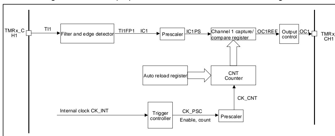
Figure 41 General-purpose Timer TMR14 Structure Block Diagram
