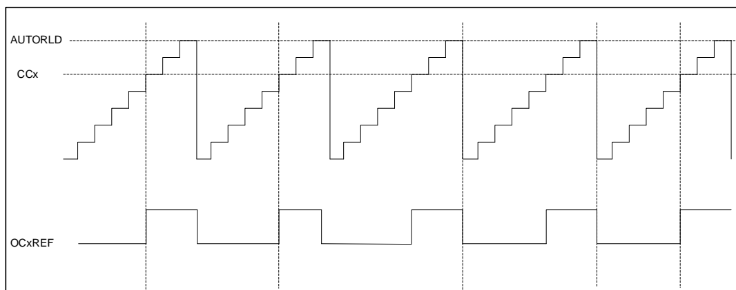
Figure 58 PWM2 Count-up Mode Timing Diagram
