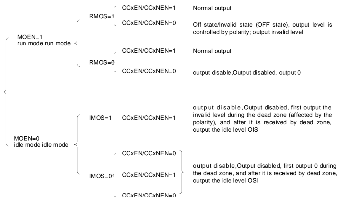
Figure 63 Register Structural Relationship Affecting Output Waveform
