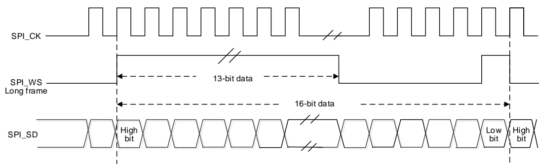
Figure 122 PCM Standard Waveform
