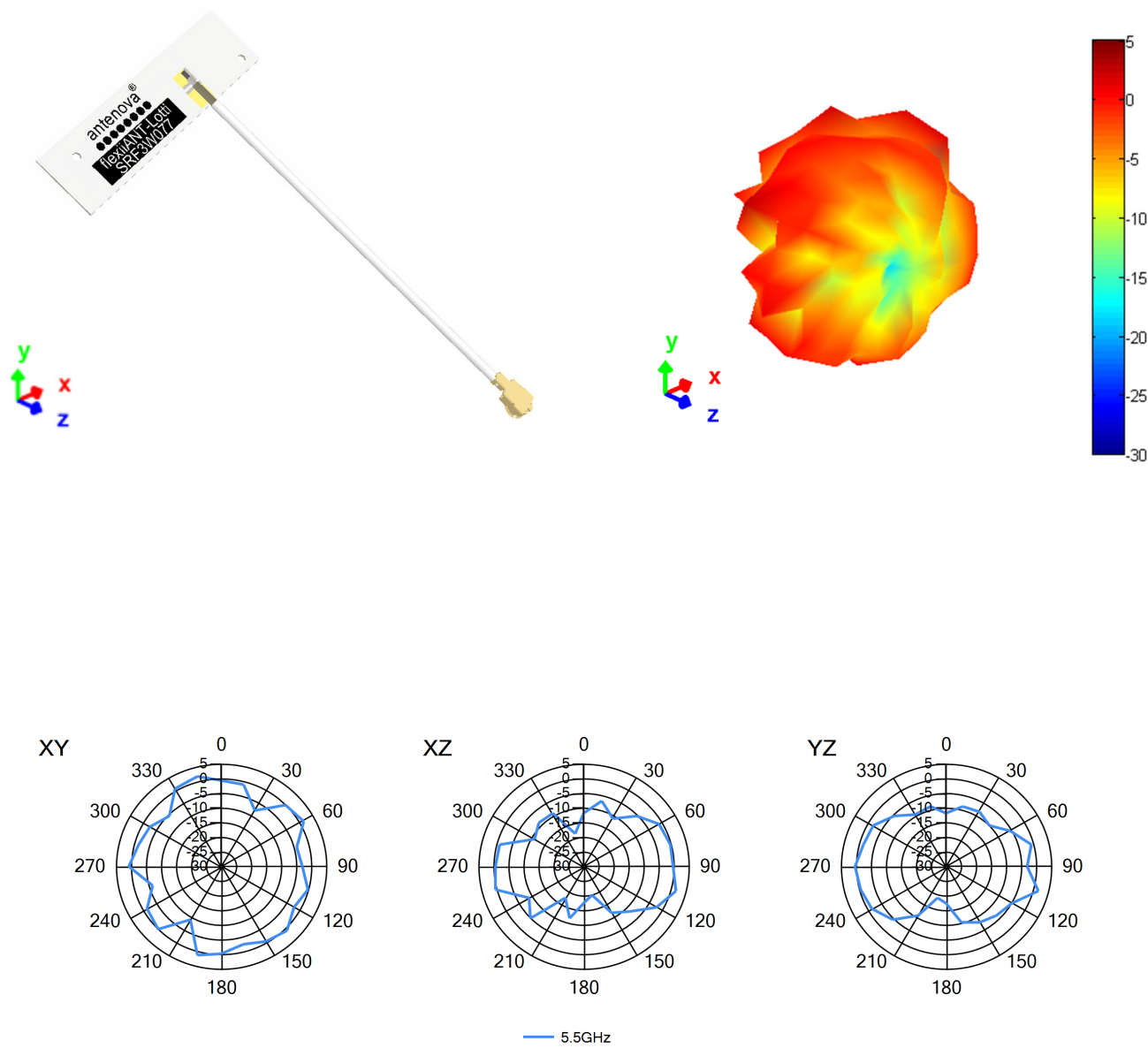
3D pattern at 5500 MHz
