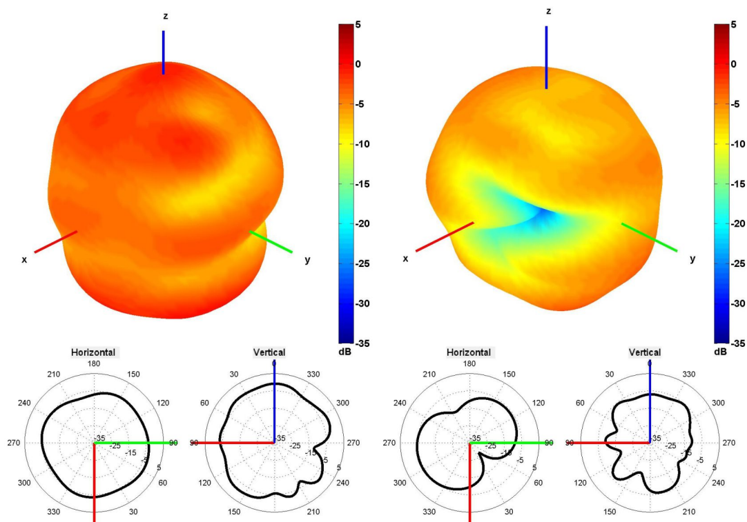
Cable 1: GNSS/L1L5
