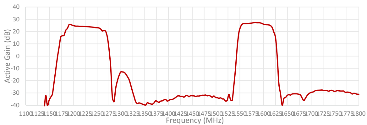
Cable 1: GNSS/L1L5
