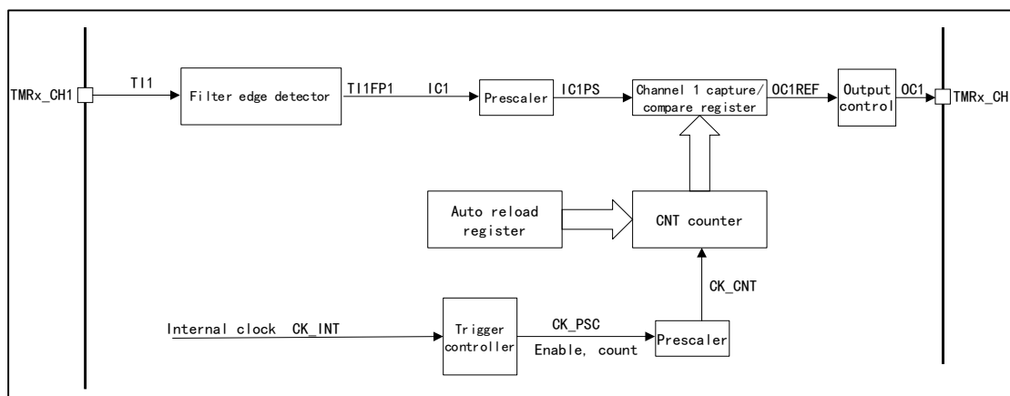
Figure 55 General-purpose Timer TMR10/11/13/14 Structure Block Diagram
