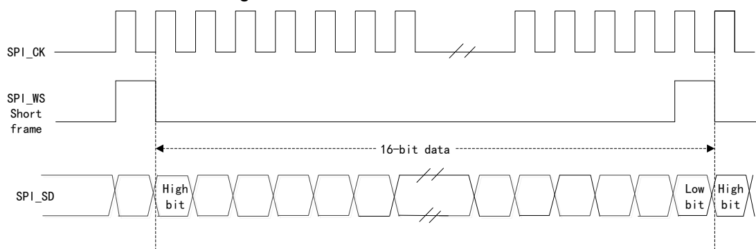
Figure 98 PCM Standard Waveform
