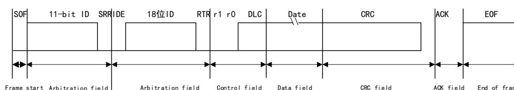
Figure 107 Extended Data Frame
