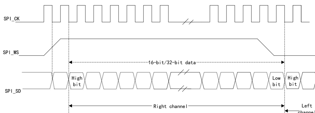
Figure 88 I2S Philips Protocol Waveform (16/32 bits)
