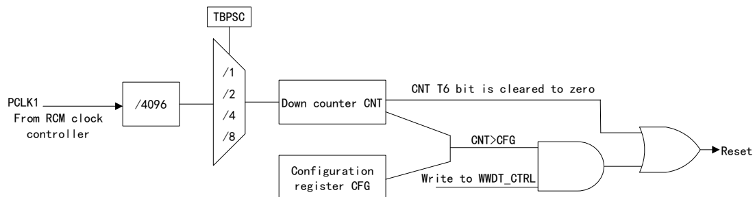
Figure 62 Window Watchdog Structure Block Diagram
