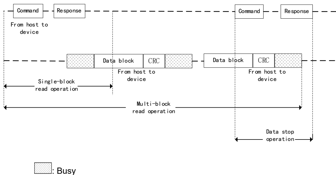
Figure 119 SDIO Data Flow Read Operation
