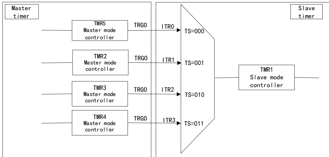
Figure 35 Timer 1 Master/Slave Mode Example
