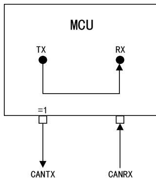
Figure 110 CAN Works in Mute Loopback Mode
