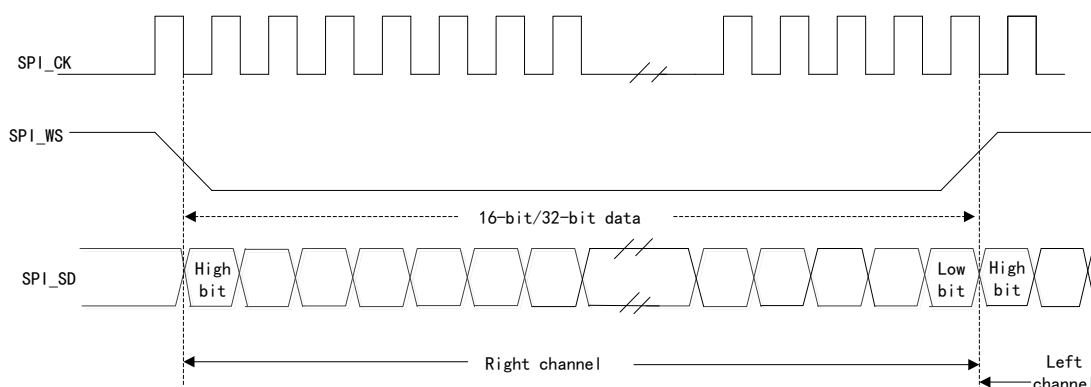
Figure 91 MSB Alignment Standard Waveform (16/32-bit data)
