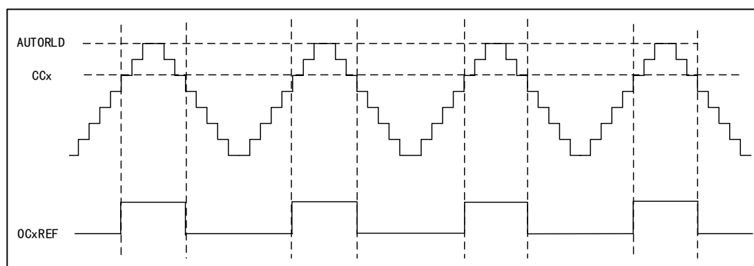
Figure 27 Timing Diagram of PWM2 Center-aligned Mode
