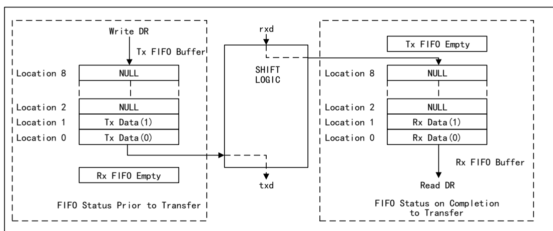
Figure 99 QSPI Transmit FIFO State in Transmitting and Receiving State
