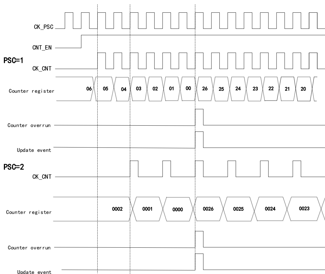
Figure 19 Timing Diagram of Count-down Mode when Division Factor is 1 or 2
