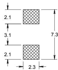
Recommended layout for solder pads
