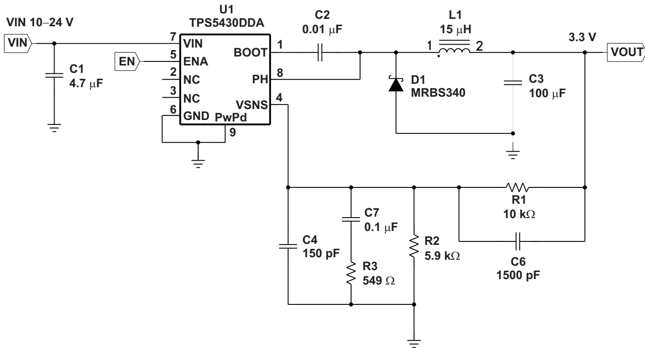
Figure 14. Ceramic Output Filter Capacitors Circuit
