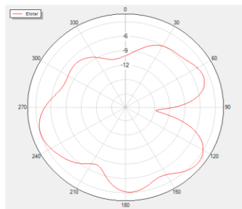
Theta=90 Freq=830MHz
