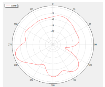
Theta=90 Freq=900MHz
