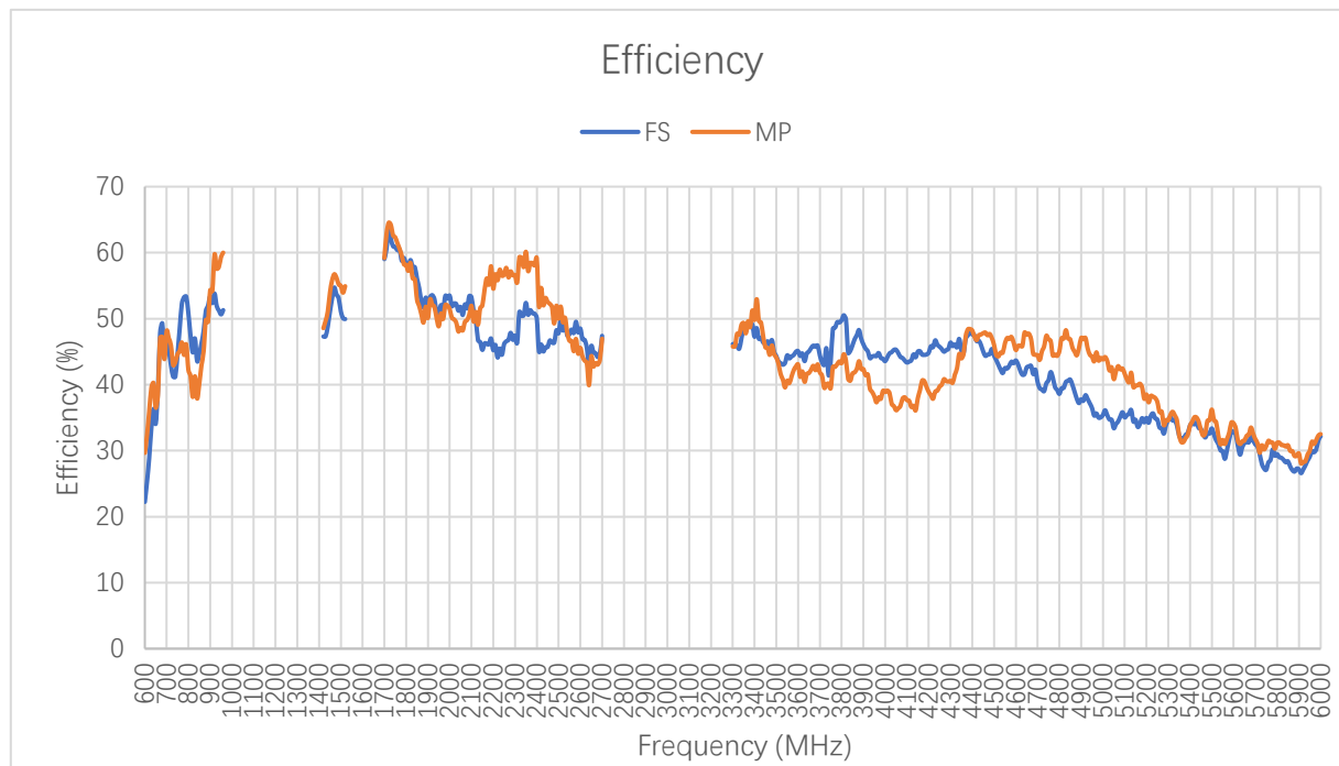
Efficiency (%)
