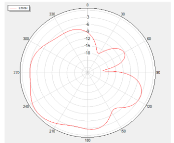
Theta=90 Freq=710MHz
