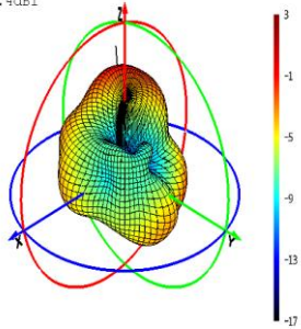
Phi=0 Freq=630MHz
