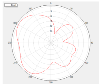
Phi=90 Freq=710MHz
