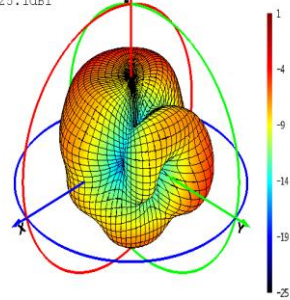
Phi=0 Freq=710MHz
