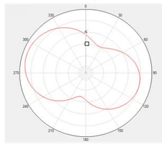
Theta=90 Freq=1602MHz
