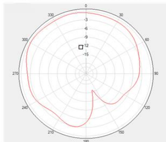
Phi=90 Freq=1176MHz
