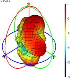
Phi=0 Freq=2140MHz
