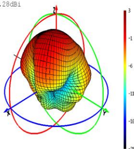
2600 MHz
