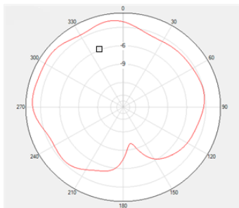
Phi=90 Freq=1602MHz
