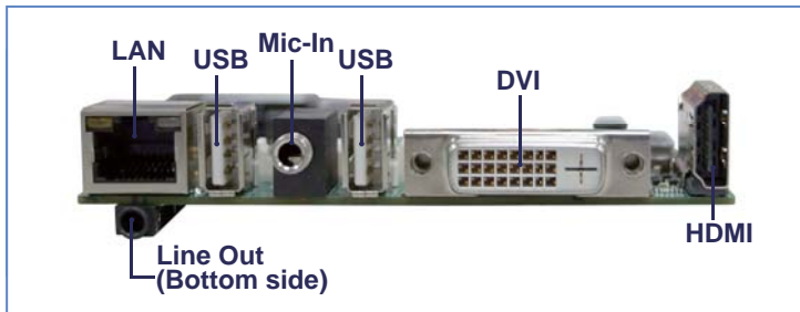
21260A-DH26-00 Rear I/O
