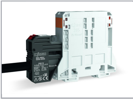
Installation via jumper slot
