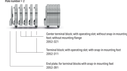
Example of a 5-pole terminal strip; with operating slot; with snap-in mounting foot
