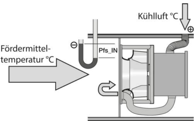
Fig. 1: Cooling air supply of the encapsulated RadiPac fan
