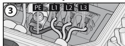
Fig. 3: Connecting wires to terminals
