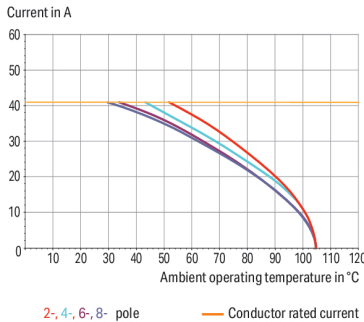
Derating Curve 1-conductor female connector (831-11xx) with THT male header (831-36xx) Pin spacing: 7.62 mm / Conductor cross-section: 6 mm² "f-st" Based on: EN 60512-5-2 / Reduction factor: 0.8
