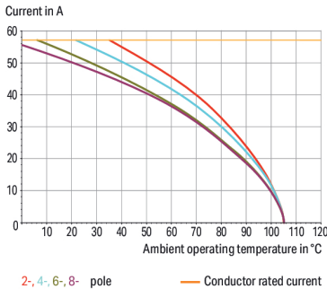
Derating Curve 1-conductor female connector (831-11xx) with 1-conductor male connector (831-12xx) Pin spacing: 7.62 mm / Conductor cross-section: 10 mm² "f-st" Based on: EN 60512-5-2 / Reduction factor: 0.8
