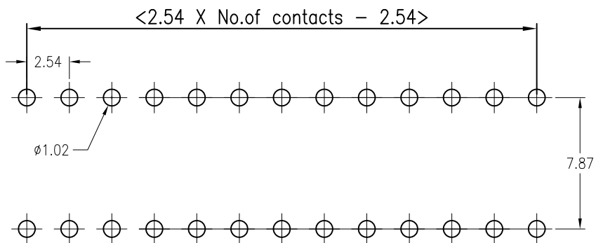
Recommended P.C. Board Hole Layout
