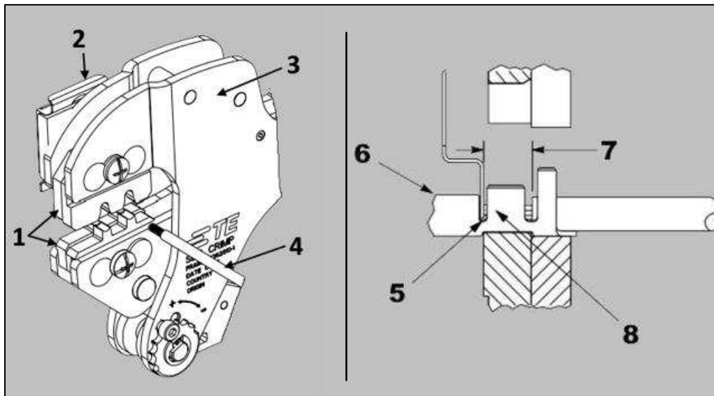
Figure 2: Crimping
