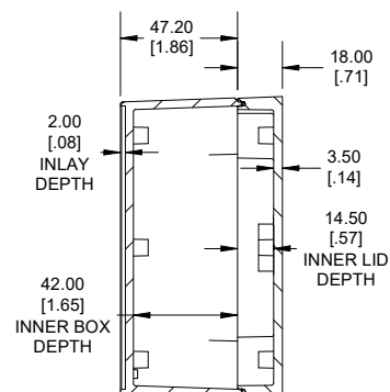
SECTION B-B SIDE VIEW
