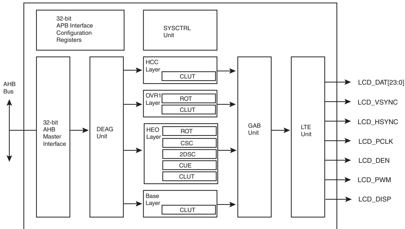
Figure 46-1. Block Diagram
