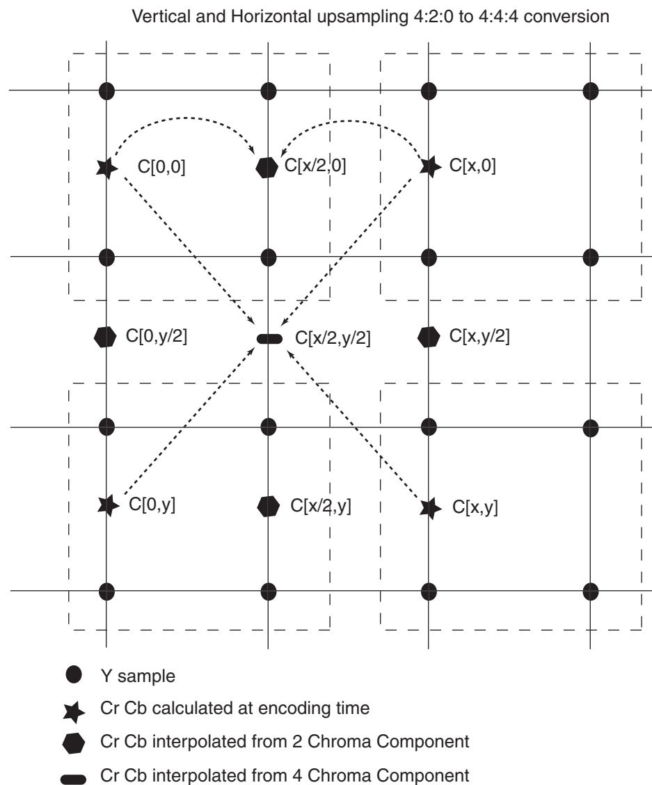
Figure 46-2. 4:2:2 Upsampling Algorithm
