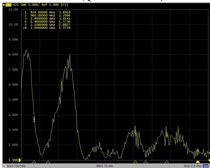
VSWR (Quad Band + WiFi)
