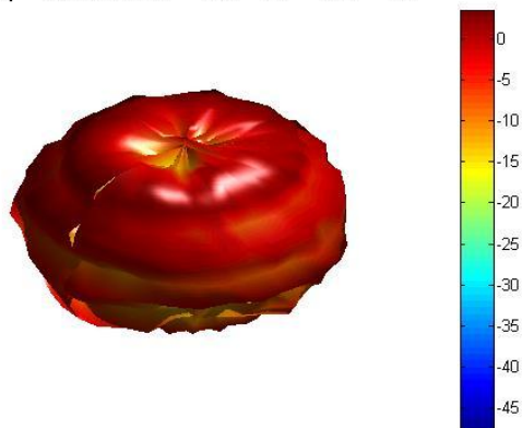
3D radiation pattern at 2.1GHz Freq = 2.104GHz Az= 45 EL= 45
