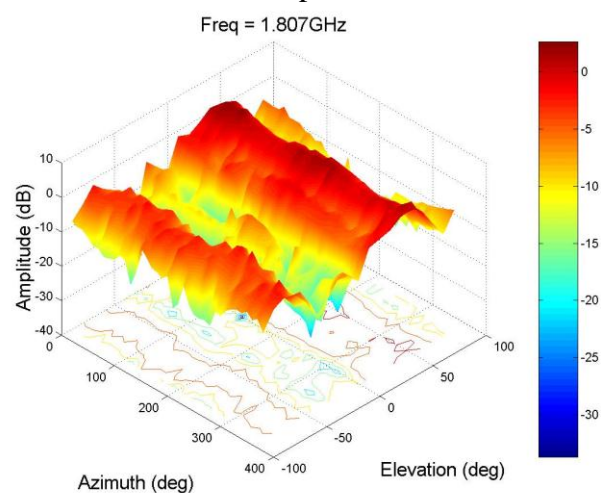
Plane radiation pattern at 1.8GHz
