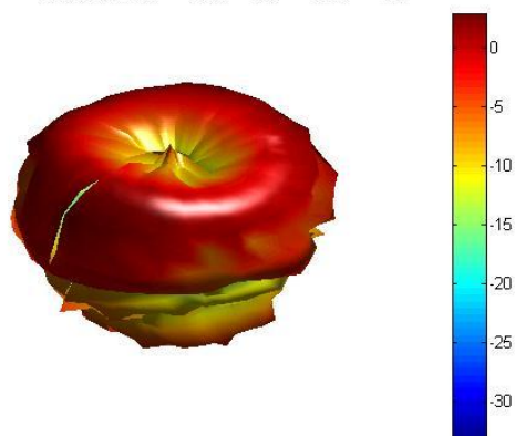
3D radiation pattern at 1.8GHz Freq = 1.807GHz Az= 45 EL= 45
