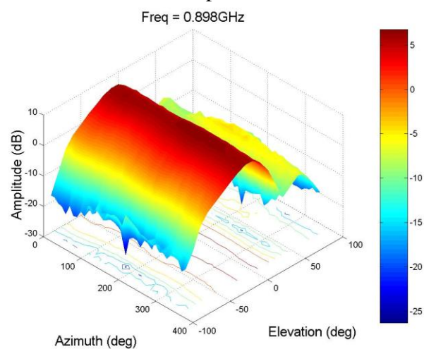
Plane radiation pattern at 900MHz
