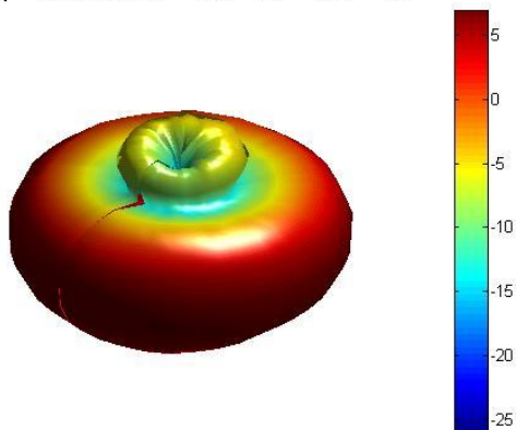
3D radiation pattern at 900MHz Freq = 0.898GHz Az= 45 EL= 45
