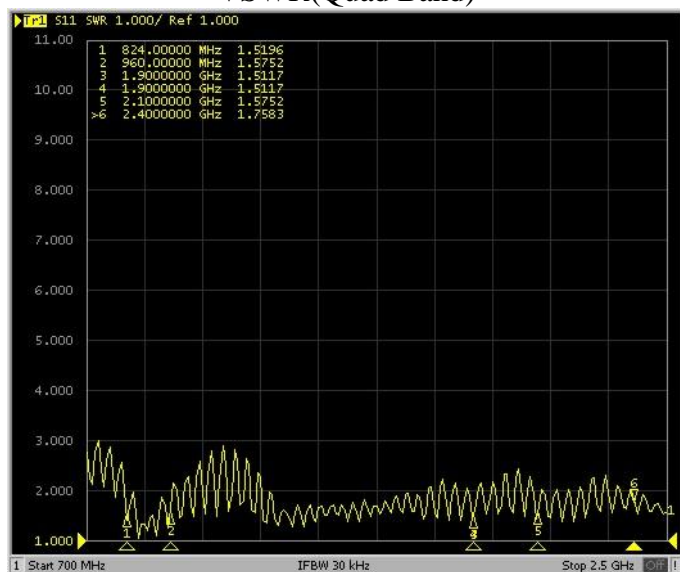
VSWR(Quad Band)
