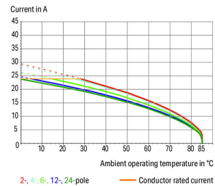
Derating Curve 1-conductor female connector (231-102/026-000) with THT male header (231-432/001-000) Pin spacing: 5 mm / Conductor cross-section: 2.5 mm 2 *F-st* Based on: EN 60512-5-2 / Reduction factor: 0.8
